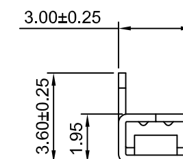
SEC:C-C
